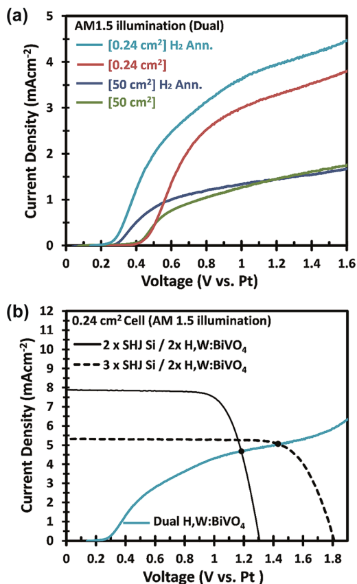
Fig. 9 (a) J - V curves comparing the effects of hydrogen annealing on the small and large area dual-CoP i /W:BiVO 4 photoanodes in 0.1 M KP i (small area) or 2.0 M KP i (large area) buffer. Large area samples are with Ni lines. (b) J - V curves of a small area 2 SHJ PV (black line) and the 3 SHJ PV (dashed black line) with dual-CoP i /H,W:BiVO 4 photoanodes as the front windows, and the small area dual-CoP i /H, W:BiVO 4 photoanode, measured in 0.1 M KP i buffer.
