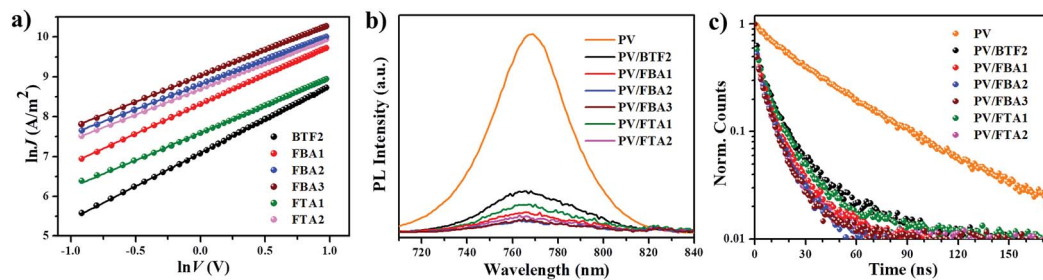
Fig. 4 (a) The hole injection characteristics measured by the SCLC method based on a device structure of ITO/PEDOT:PSS/HTM/MoO x (10 nm)/Ag. (b) Steady PL spectra and (c) time-resolved PL spectra of bare perovskite (PV) films and bi-layered perovskite films capped with different fluoranthene-cored HTMs.
