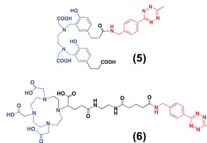
Fig. 2 (A) Structure of HBED-CC-tetrazine ( \mathbf{5} ) and DOTA-GA-tetrazine ( \mathbf{6} ).
