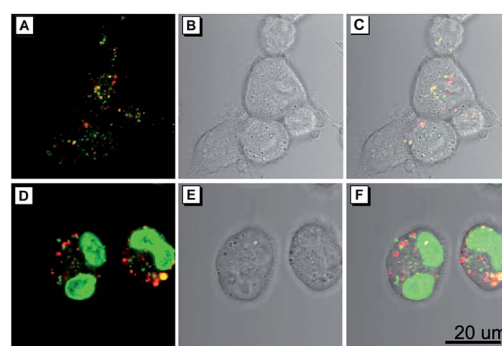
Fig. 7 Cell fusion of COS-7 cells induced by 50% polyethylene glycol (PEG), and visualized through fluorescence imaging of TTG and TTNIR. (A) Confocal image and (B) bright-field of mixed cells respectively stained with TTG and TTNIR. (C) Merged images of panels (A) and (B). (D) Confocal image and (E) bright-field of mixed cells respectively stained with TTG, TTNIR and Hoechst 33258. (F) Merged images of panels (D) and (E). For TTG, \lambda_{\text{ex}} : 405 nm (1% laser power), \lambda_{\text{em}} : 425–540 nm. For TTNIR, \lambda_{\text{ex}} : 560 nm (6.5% laser power), \lambda_{\text{em}} : 600–740 nm. For Hoechst 33258, \lambda_{\text{ex}} : 405 nm (3.5% laser power), \lambda_{\text{em}} : 425–540 nm. Concentrations: TTG (500 nM), TTNIR (2 \mu\text{M} ), Hoechst 33258 (2.5 \mu\text{M} ). Scale bar = 20 \mu\text{m} .
