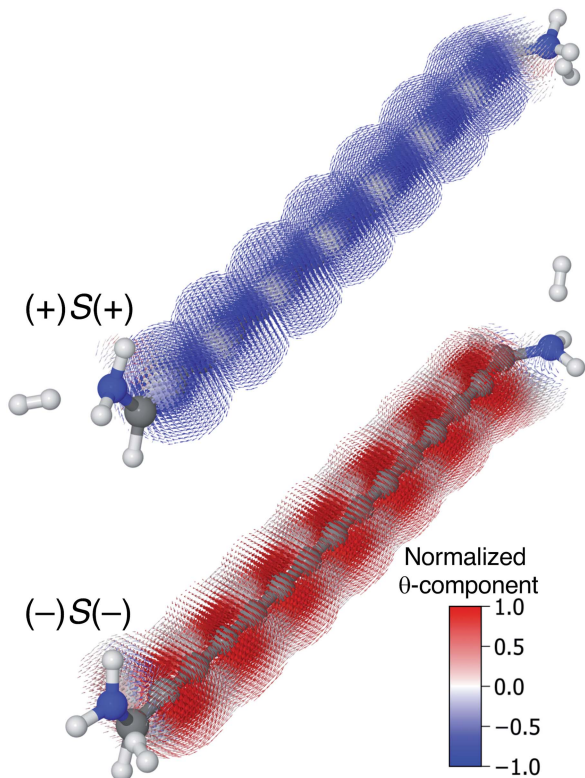
Fig. 10 Current density calculated at the Fermi energy for the (+)S(+) and (–)S(–) conformations of 1,5-diamino-[14]cumulene; the 15-carbon cumulene with helical \pi -orbitals. The vector field is calculated on a high-density grid and coloured by the \theta -component.
