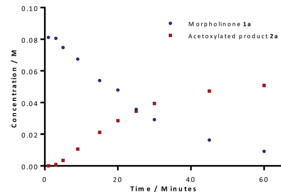
Fig. 1 Reaction profile for the acetoxylation of morpholinone 1a .
