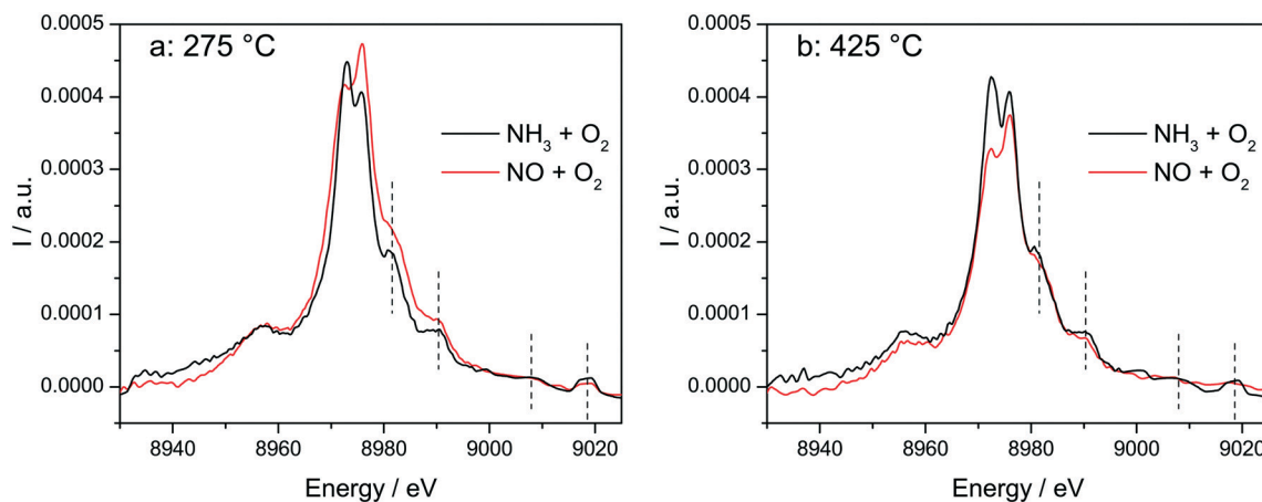
Fig. 10 In situ vtc-XES measured on Cu-1.2 at (a) 275 °C and (b) 425 °C. Conditions: 1000 ppm NO or 1000 ppm NH 3 , 10% O 2 , 1.5% H 2 O, balance He, GHSV 200 000 h -1 .
