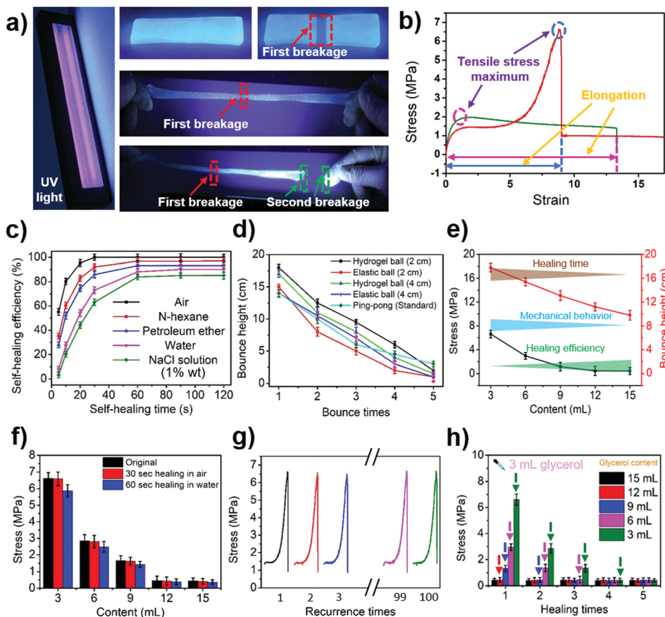
Fig. 2 (a) Self-healing performance photos of the hydrogel under UV light. (b) Typical tensile stress–strain curves of different glycerol contents contained within the hydrogels. (c) Relationship between the self-healing efficiency and healing time of the hydrogel in different media. (d) Bounce height–time curves of different balls. (e) Relationship between the properties of the hydrogel and the glycerol content in the hydrogel. (f) Tensile stress–glycerol content curves of the hydrogel in different stages (original, self-healed) and different media. (g) Relationship between the pressure remodeling times and tensile properties of hydrogels. (h) Performance diagram of hydrogels obtained by adding glycerol at two different time periods (during preparing, during remodeling).
