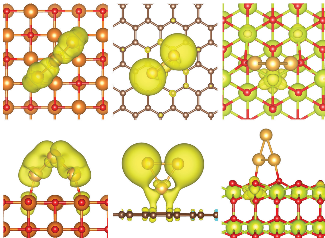
Fig. 9 Iso-surfaces of the highest occupied band of Au 3 /MgO (left), Au 3 /C (centre), and Au 3 /CeO 2 (right); iso-value of 0.001 e -3 .
