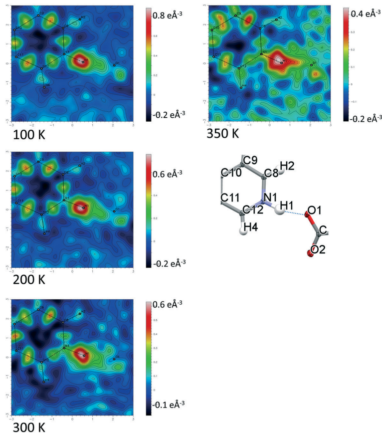
Fig. 12 Fourier difference electron density maps showing the electron density associated with the H-atom in the N^+-H\cdots O^- SSHB in 8 over the 100 to 350 K temperature range.
