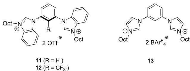
Fig. 3 Structures of reference compounds.
