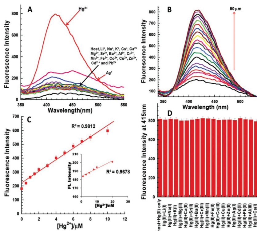
Fig. 15 (A) Changes in the emission profile of nanoaggregates 13 (10 \mu M ) in water upon the addition of 50 \mu M of a particular metal nitrate salt; (B) changes in the emission profile of nanoaggregates 13 (10 \mu M ) upon the successive addition of Hg^{2+} (0–50 \mu M ); (C) linear regression graph between the concentration of added mercury ions (0–10 \mu M ) and increase in the fluorescence intensity of nanoaggregates 13 (25 \mu M ). Inset: Linear regression plot of nanoaggregates 13 (10 \mu M ) and addition of Hg^{2+} in the range of 0–20 nM; (D) influence of other metal ions on Hg^{2+} -based changes in the emission profile of nanoaggregates 13 . Adapted with permission from ref. 71. Copyright 2014 the Royal Society of Chemistry.
