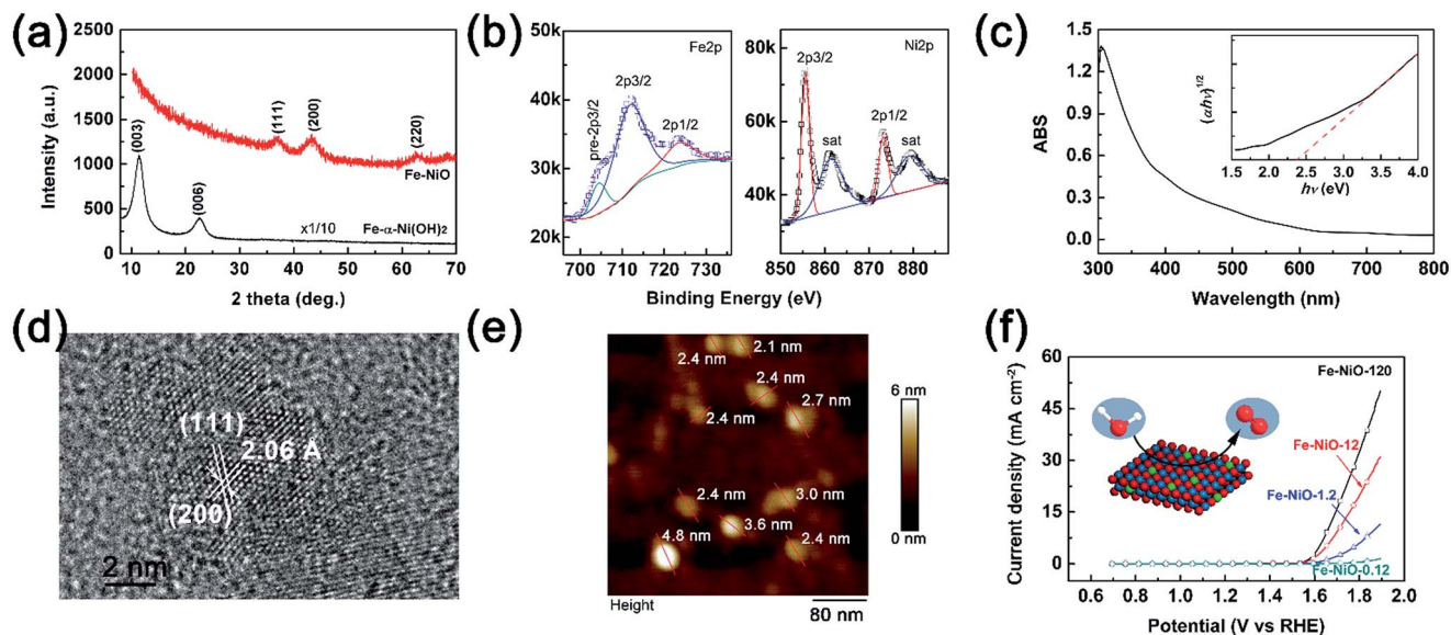
Fig. 1 (a) XRD patterns of the Fe-doped Ni(OH) 2 precipitate (black curve at bottom) and Fe-doped NiO (red curve on the top); (b) XPS spectra of the Fe-NiO film (left: Fe2p; right: Ni2p); (c) UV-vis absorption spectrum of the Fe-NiO film, the inset was the Tauc plot of indirect band estimation; (d) HR-TEM image of the Fe-NiO nanosheet; (e) AFM height image of the Fe-NiO nanosheets; (f) J - V curves of the Fe-NiO nanosheets on FTO prepared with various concentrations in a 1 M NaOH electrolyte, and a scanning rate of 20 mV s -1 .
