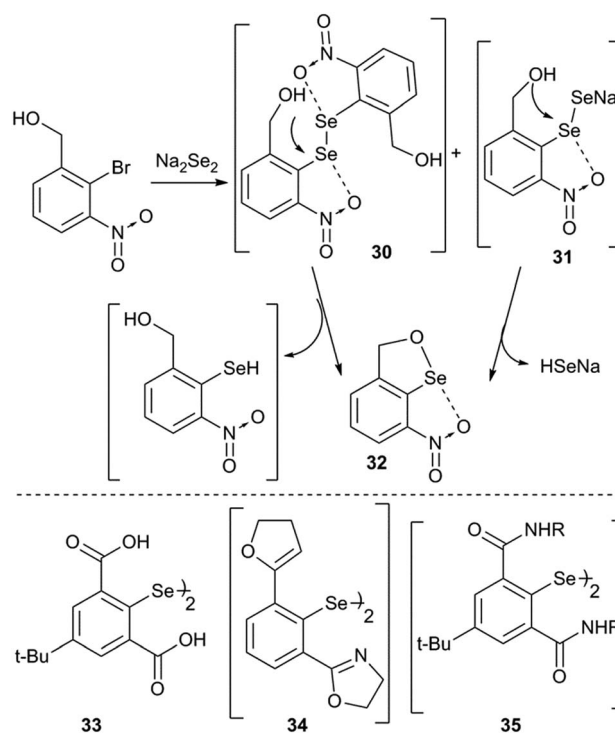
Fig. 10 Top panel shows the intramolecular addition–elimination reaction of diselenide motifs ( 30 and 31 ). The bottom panel shows the structures of other diaryl diselenide/diaryldiselenide intermediates.
