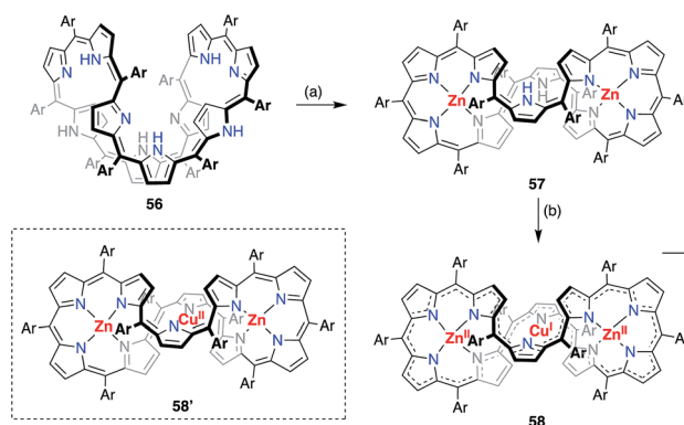
Fig. 18 Synthesis of the decaphyrin Zn(II)–Cu(I)–Zn(II) complex 58 . (a) 5 equiv. \text{Zn}(\text{OAc})_2 \cdot 2\text{H}_2\text{O} , 5 equiv. \text{NaOAc} , \text{MeOH} , reflux, 2 h, 61%; (b) 10 equiv. \text{Cu}(\text{OAc})_2 , 10 equiv. \text{NaOAc} , \text{MeOH} , rt, 4 h, 72%. Ar = pentafluorophenyl.
