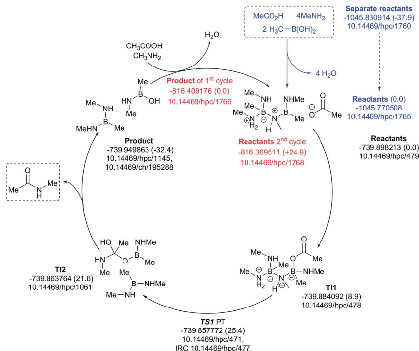
Fig. 12 Catalytic cycle involving four amines (data 29 sub-collection DOI: 10.14469/hpc/1728; the labels have the same meaning as in Fig. 9). All DOIs in this figure are available as clickable links (final paginated PDF only).
