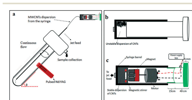
Fig. 1 Laser-VFD fabrication of carbon dots (CDs) under continuous flow. (a) Schematic of the vortex fluidic device (VFD). (b) Illustration of an unstable dispersion of MWCNTs in aqueous H 2 O 2 in a normal syringe. (c) Magnetic-assisted mixing in a syringe for delivering a uniform dispersion of MWCNTs to the base of the rapidly rotating borosilicate glass tube (20 mm O.D. diameter).
