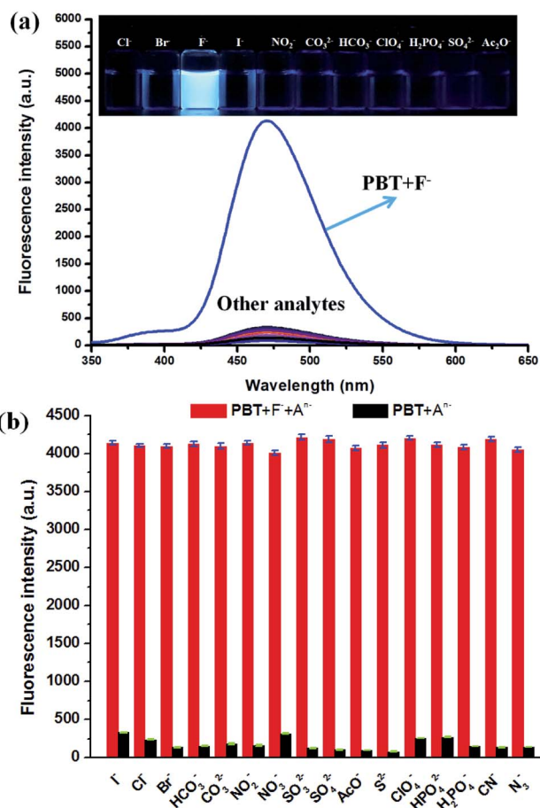
Fig. 6 (a) Fluorescence spectra of PBT in the presence of various anions. [PBT] = 10 \mu\text{M} , [An^-] = 20 \mu\text{M} , in a mixture of THF and Tris buffer solution (pH 8.0), (1 : 9, v/v), \lambda_{\text{ex}} = 335 \text{ nm} , \lambda_{\text{em}} = 470 \text{ nm} . Inset: direct observation of fluorescence emission difference of the probe PBT ( 10 \mu\text{M} ) under UV irradiation (365 nm) in the presence of different anions. Left to right: Cl^- , Br^- , I^- , F^- , NO_2^- , CO_3^{2-} , HCO_3^- , ClO_4^- , H_2PO_4^- , SO_4^{2-} and AcO^- . (b) The selectivity of PBT in the presence of various anions.
