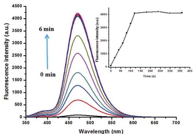
Fig. 5 Time course of the signaling of PBT by F^- [PBT is 10 \mu\text{M} , [F^-] is 20 \mu\text{M} ], in a mixture of THF and Tris buffer solution (pH 8.0), (1 : 9, v/v), \lambda_{\text{ex}} = 335 \text{ nm} , \lambda_{\text{em}} = 470 \text{ nm} . Inset: the response curve of fluorescence intensity of PBT with F^- depending on the various time.
