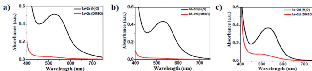
Fig. 2 UV-Vis absorption spectra of the 1 : 1 blend of (a) 1a + 2a , (b) 1d + 2d and (c) 1a + 2d (black in H_2O and red in DMSO) at 20\ 000 \mu\text{M} .
