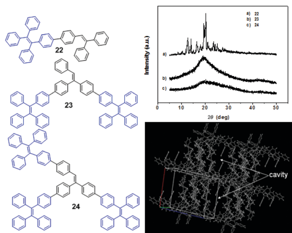
Fig. 3 (top) Wide-angle X-ray diffraction curves of the as-synthesized samples 22 – 24 ; (bottom) molecular packing of 22 in the single crystal state (wireframe style). (left) The molecular structures of compounds 22 – 24 . Reproduced with permission from ref. 45. Copyright 2011 Wiley-VCH.
