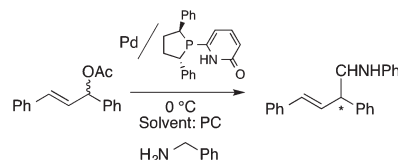
Scheme 29 Pd-Catalyzed asymmetric alkylation using a chiral phosphine catalyst.
