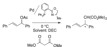
Scheme 28 Pd-Catalyzed asymmetric alkylation in DEC.
