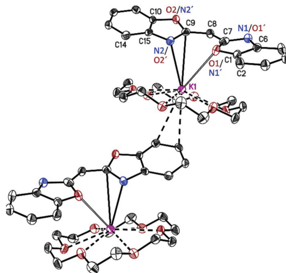
Fig. 3 Polymeric structure of [[\{\text{NCOC}_6\text{H}_4\}_2\text{CH}\text{K}(18\text{-crown-6})]_n ( 3 ). Anisotropic displacement parameters are depicted at the 50% probability level. Hydrogen atoms are omitted for clarity. Structural data are given in Table 1 and the Experimental.
