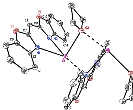
Fig. 2 Polymeric structure of [[\{\text{NCOC}_6\text{H}_4\}_2\text{CH}\text{K}(\text{thf})]_n ( 2 ). Anisotropic displacement parameters are depicted at the 50% probability level. Hydrogen atoms and the positional disorder are omitted for clarity. Structural data are given in Table 1 and the Experimental section.
