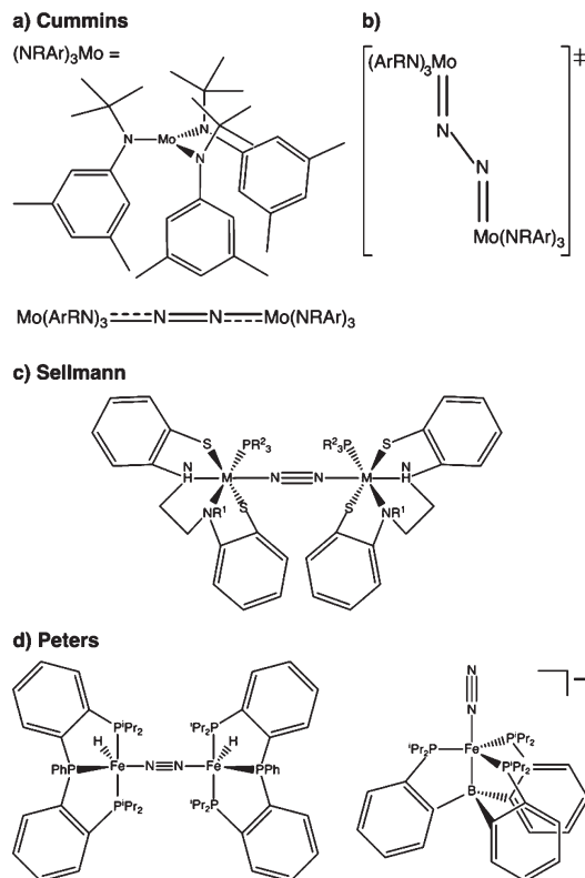
Fig. 2 Thermal dinitrogen activation complexes: (a) Cummins, (b) zig-zag transition state relevant to the Cummins complex, (c) Sellmann, (d) Peters: left [P_2^{P^Ph}]FeH_2(\mu-N_2) , right [P_3^{B^Fe}(N_2)]^- .
