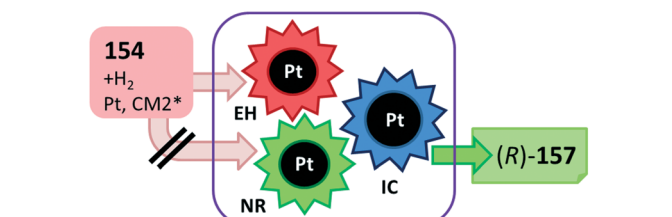
Scheme 46 Cascade EH, NR and IC of 2-nitrophenylpyruvates over chirally modified supported Pt catalyst. 203,204
