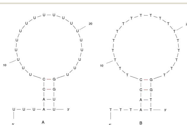
Fig. 1 The ideal structure of the (A) RNA and (B) DNA hairpin loop secondary structural motifs. Results were taken from the mfold web server. 24
