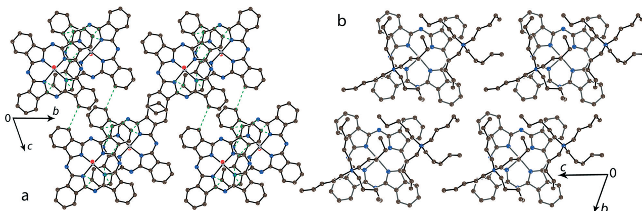
Fig. 4 (a) View of the phthalocyanine layer composed of the \pi -stacking [\{\text{Ti}^{\text{IV}}\text{O}(\text{Pc}^{3-})\}]_2 dimers in 4 . Short van der Waals C,N...C,N contacts are shown by green dashed lines. (b) Projection of the \text{Pent}_4\text{N}^+ layer on the phthalocyanine layer. Only one phthalocyanine from the dimer is shown (bonds are shown in grey).
