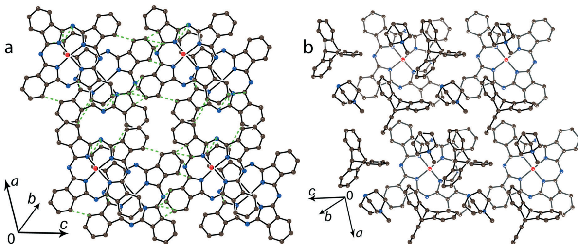
Fig. 10 (a) View of the phthalocyanine layer composed of the \pi -stacking [\{\text{Ti}^{\text{IV}}\text{O}(\text{Pc}^{3-})\}^-]_2 dimers in 12 . Short van der Waals C...C,N contacts are shown by green dashed lines. (b) Projection of the (MDABCO + )-TPC layer on the phthalocyanine layer. Only one phthalocyanine from the dimer is shown (bonds are shown in grey).
