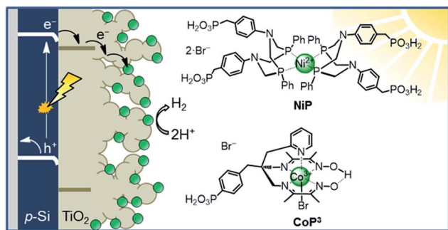
Fig. 1 Schematic diagram of PEC \text{H}_2 evolution with the \text{Si|mesoTiO}_2|\text{catalyst} photocathode and chemical structures of the immobilised catalysts NiP and CoP 3 .
