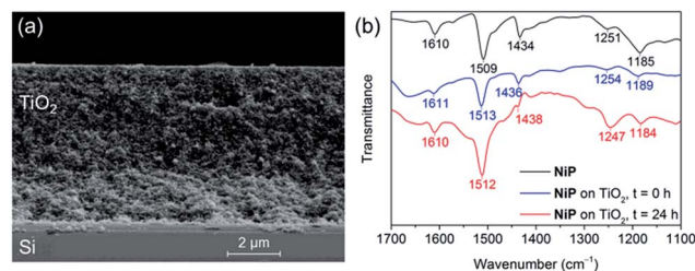
Fig. 2 (a) SEM cross-section image of a \text{Si|mesoTiO}_2 electrode. (b) ATR-FTIR spectra of NiP (black), \text{Si|mesoTiO}_2|\text{NiP} before (blue) and after (red) 24 h CPP.
