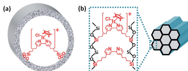
Scheme 4 Schematic of (a) IrCp*-Gbpsy-NT and (b) IrCp*-BPy-SBA-15.
