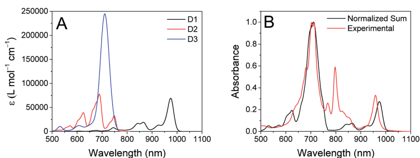
Fig. 8 Left: Calculated vibronic transitions from the ground state to the D1 (black), D2 (red) and D3 (blue) states of PDI 1- . Right: Sum of the three calculated vibronic spectra (black) compared to the experimentally determined spectrum of PDI 1- , normalized to the maximum value.
