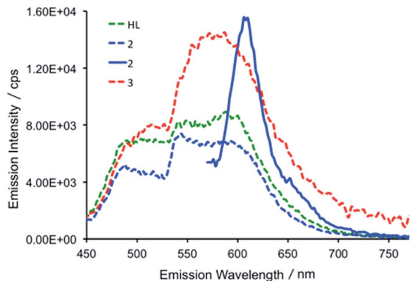
Fig. 6 Emission spectra of HL (green dashed trace), 2 (blue dashed trace) and 3 (red dashed trace) following excitation at 425 nm and the emission spectrum of 2 (full blue line) following 550 nm excitation (298 K, THF). The relative intensities of HL, 2 and 3 are arbitrary with respect to each other.
