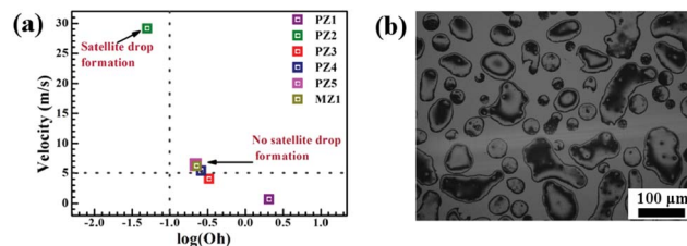
Fig. 8 PZ3 ink drops deposited in single pass using the commercial inkjet printer. Drops deposited do not show any satellite drop formation. The horizontal and vertical dotted lines represent the boundary between the satellite drop and no satellite drop regions. (a) \log(\text{Oh}) vs. velocity plot for PZ3, PZ4, PZ5 and MZ1 inks lie at the border of no satellite drop formation. 45 (b) Few merged drops can be seen along with regular droplets. There are also some smaller size drops and satellite drop formation cannot be completely ruled out.
