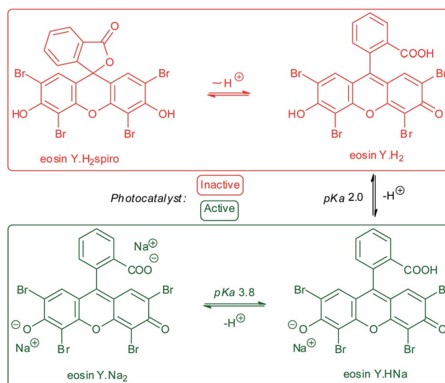
Scheme 2 Acid–base behaviour of eosin Y.
