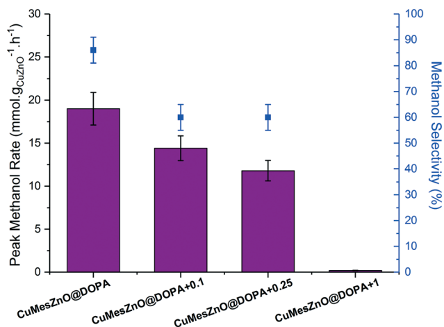
Fig. 5 Peak MeOH rates and selectivity of CuMesZnO@DOPA+x catalysts prepared varying amounts [DOPA] − ligand. Reaction conditions: 210 °C, 50 bar, H 2 :CO 2 molar ratio of 3:1, 10.8 L syngas mmol Cu+Zn −1 h −1 in mesitylene.
