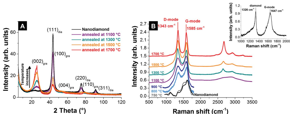
Fig. 5 (A) X-ray diffractograms of nanodiamond and carbon onions synthesized at different temperatures in an argon atmosphere. 32 (B) Raman spectra of nanodiamond-derived carbon onions synthesized in argon measured with a 532 nm laser (recorded using 0.2 mW, 30 accumulations, and 10 s acquisition time; for pristine nanodiamonds and nanodiamonds annealed at 750–900 °C the spectra were only recorded using 1 accumulation to avoid laser-induced heating and were baseline-corrected). 32 The inset shows the Raman spectrum of nanodiamonds measured with a 325 nm UV-laser. 110
