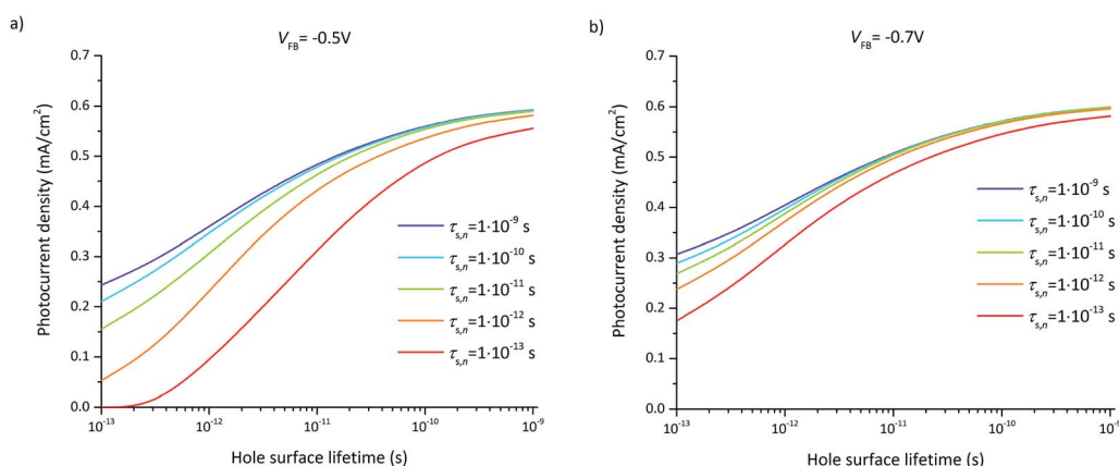
Fig. 11 Photocurrent density at 0.3 V vs. RHE as a function of the hole surface lifetime for various electron lifetimes ( \tau_{s,n} = 10^{-9} , 10^{-10} , 10^{-11} , 10^{-12} , 10^{-13} s) and two flatband potentials: (a) V_{FB} = -0.5 V vs. RHE, and (b) V_{FB} = -0.7 V vs. RHE.
