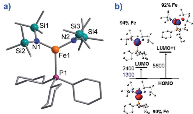
Fig. 10 (a) Molecular structure of [\text{Fe}(\text{N}(\text{TMS})_2)_2(\text{PCy}_3)] , ( \text{TMS} = \text{SiMe}_3 , \text{Cy} = \text{cyclohexyl} ) ( 8 ). Colour code: orange (Fe), plum (P), teal (Si), blue (N), grey (C). Hydrogen atoms omitted for clarity. (b) TD-DFT calculated excited states and \beta -spin molecular orbitals (MOs). The energies of the excited states and the metal contribution to the MOs are also shown. Reprinted with permission from ref. 34. Copyright (2011) American Chemical Society.
