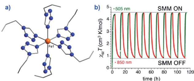
Fig. 8 (a) Molecular structure of [Fe(1-ptz) 6 ] 2+ [(BF 4 ) 2 ] - (2). Colour code: orange (Fe), blue (N), and grey (C). Hydrogen atoms omitted for clarity. (b) Excitation and de-excitation cycling between the HS and LS configuration of 2, represented as a variation in the \chi_M T product at 10 K, under a 5000 Oe field. Reprinted with permission from ref. 28. Copyright (2013) American Chemical Society.
