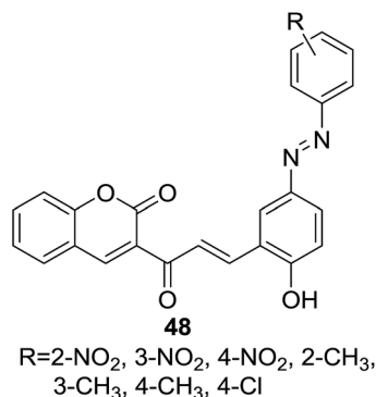
Fig. 11 Coumarin–chalcone hybrids containing an azo-linkage.
