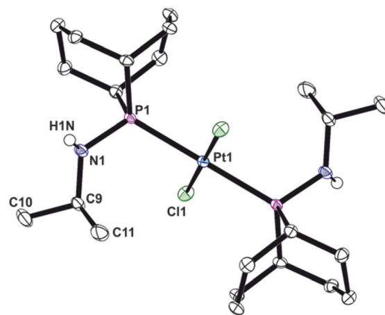
Fig. 1 Crystal structure of trans -[ \text{PtCl}_2(\text{PhobPNH}^i\text{Pr})_2 ] ( 1b ). All hydrogen atoms have been omitted for clarity. Selected bond lengths (Å) and angles (°): Pt(1)–P(1) 2.3241(10), Pt(1)–Cl(1) 2.3102(8), P(1)–N(1) 1.6594(16), Pt(1)–P(1)–N(1) 109.40(6).
