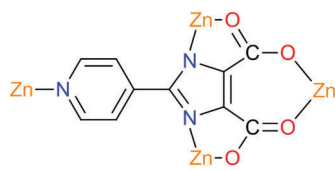
Fig. 12 Section of the structure of [\text{Zn}_2(\text{pid})(\text{H}_2\text{O})\text{Cl}]_n . 78
