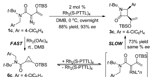
Scheme 2 Donor–acceptor cyclopropanes are reaction intermediates in metal carbene formation.
