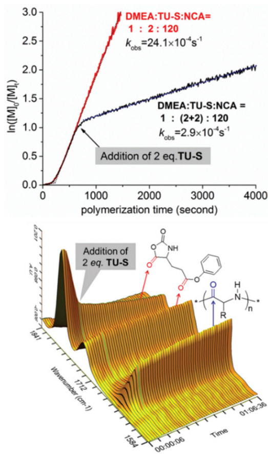
Fig. 6 \ln([\text{NCA}]_0/[\text{NCA}]_t) vs. time for the ROP of Glu-NCA initiated by DMEA/TU-S ( [\text{M}] = 0.19 \text{ M} , [\text{Glu-NCA}]/[\text{TU-S}]/[\text{DMEA}] = 120/(2 + 2)/1 , 25^\circ\text{C} , \text{CH}_2\text{Cl}_2 ) and corresponding 3D kinetic behavior profile from in situ IR (the sampling interval of in situ IR is 10 seconds).
