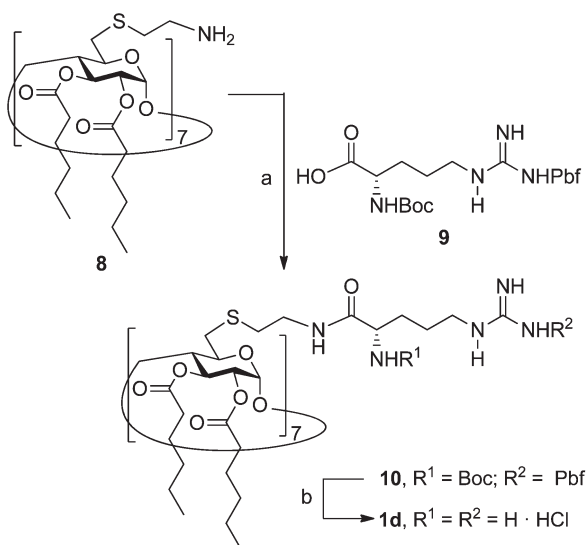
Scheme 2 Synthesis of amide-linked polyarginine \beta CD derivative 1d . Reagents and conditions: (a) HBTU, DIPEA, DCM, rt, 12 h, 68%; (b) (i) 95:2.5:2.5 TFA–TIS–DCM, rt, 1 h; (ii) 0.1 M HCl, quantitative. Pbf: 2,2,4,6,7-pentamethyl-dihydrobenzofuran-5-sulfonyl. HBTU: o -(benzo-triazol-1-yl)- N,N,N',N' -tetramethyluronium hexafluorophosphate. DIPEA: Diisopropyl ethyl amine. TIS: triisopropylsilane.
