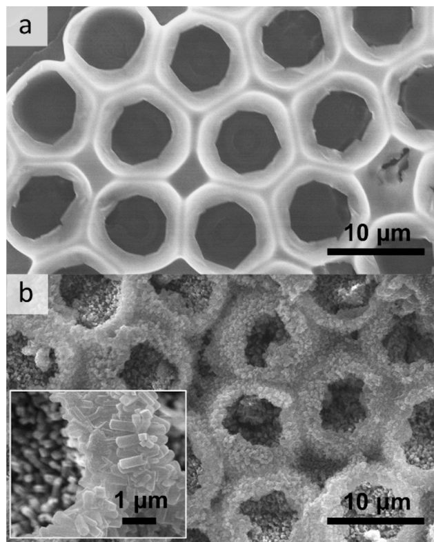
Fig. 7 FE-SEM micrographs of (a) the V_2O_5 pattern and (b) the [V(OH)ndc]_n pattern obtained after coordination replication. The SEM image in the inset is a high-magnification view of the PCP pattern.
