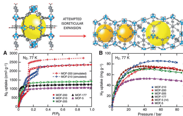
Fig. 11 (Up) The attempted isoreticular expansion of MOF-205 leads to MOF-210, and (bottom) the low-pressure N 2 isotherms (A) and high-pressure H 2 isotherms at 77 K (B) of MOF-5, -177, -200, -205, and -210. Reprinted with permission from ref. 115. Copyright 2009. American Association for the Advancement of Science.
