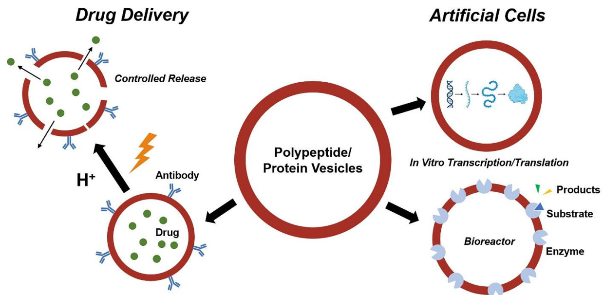
Figure 8. A schematic image of biological applications of polypeptide/protein vesicles.
