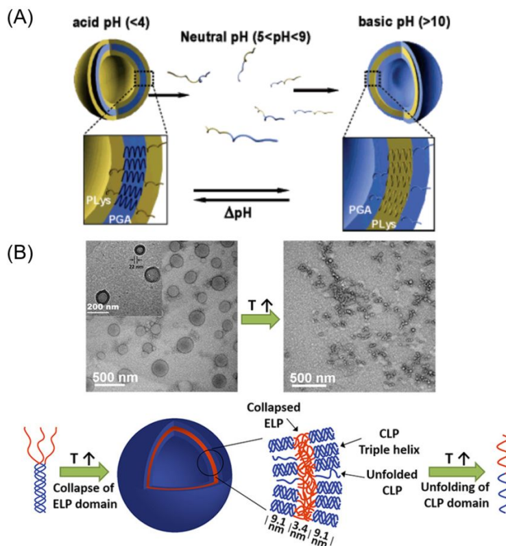
Figure 2. Self-assembly of amphiphilic polypeptides into vesicles. (A) Schematic image of the self-assembly of diblock copolymer poly(L-glutamic acid)- b -poly(L-lysine) 67 Adapted with permission from ref (67). Copyright 2005 American Chemical Society. (B) TEM images and schematic illustration of thermally induced vesicle formation from the ELP-CLP conjugates. 71 Adapted with permission from ref (71). Copyright 2015 American Chemical Society.
