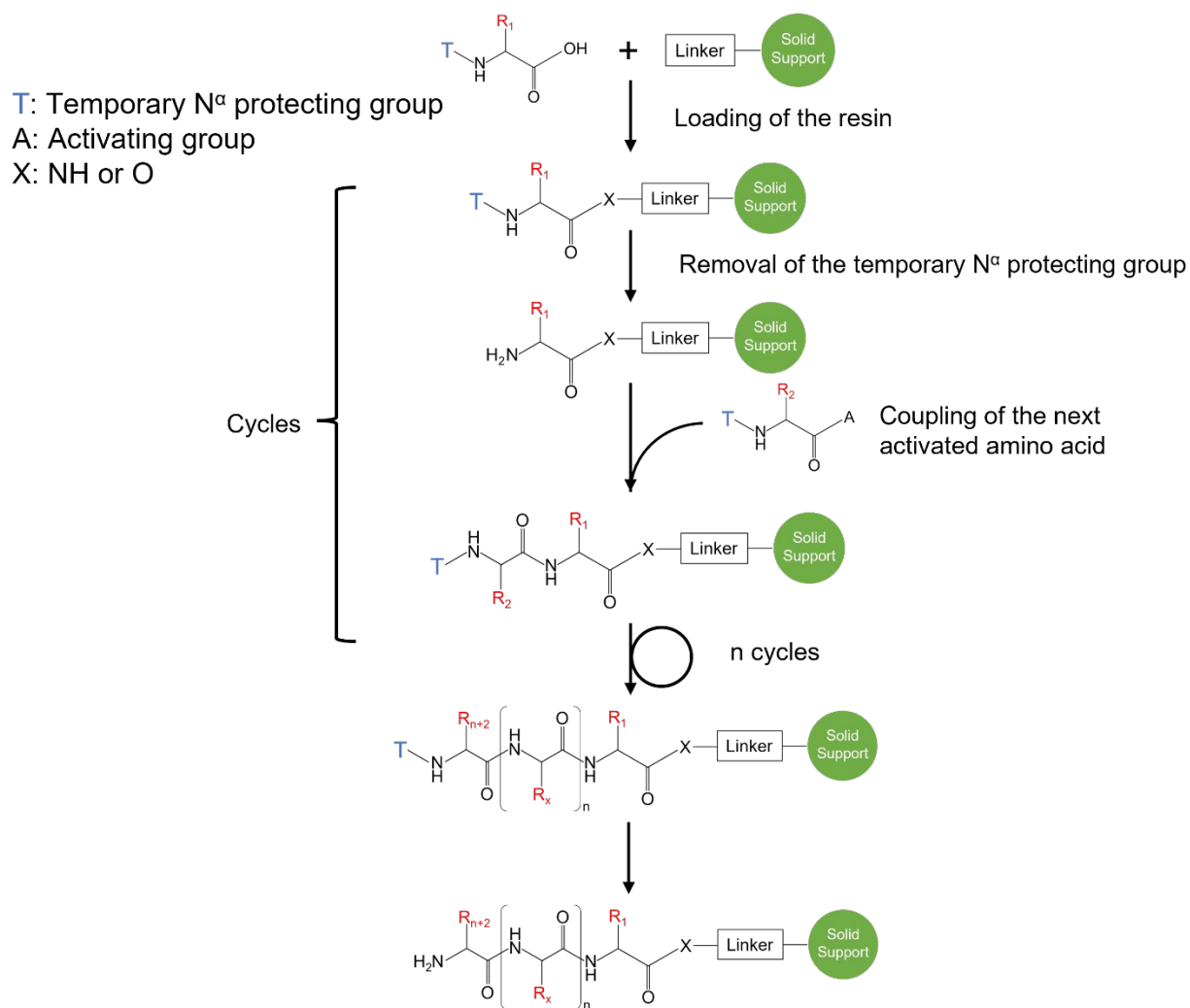
Scheme 1. Principles of solid phase peptide synthesis. 25 This scheme is created based on the ref (25) with permission. Copyright 2006 Springer Nature.
