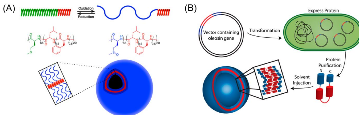
Figure 3. Polypeptide-based vesicles formed by co-solvent method. (A) Schematic illustration of structure of block copolypeptide and vesicles. 76 Adapted with permission from ref (76). Copyright 2013 American Chemical Society. (B) Schematic illustration of the expression process of recombinant oleosin protein mutants and formation of vesicles. 77 Adapted with permission from ref (77). Copyright 2012 The National Academy of Sciences
