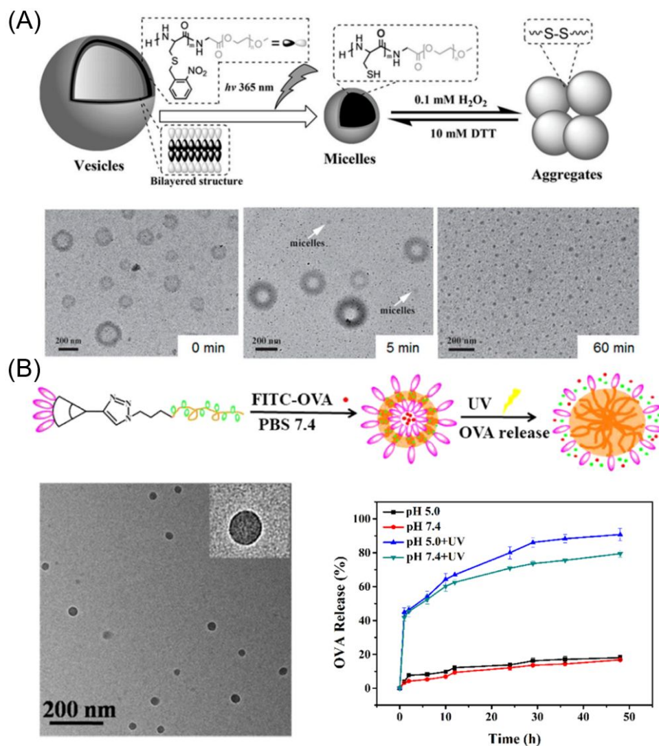
Figure 5. (A) The disassembly process of UV-light responsive polypeptide-based vesicles triggered by UV irradiation (top) and TEM images of the vesicles (bottom left), micelles (bottom middle), and aggregates (bottom right). 88 Adapted with permission from ref (88). Copyright 2014 Wiley-VCH Verlag GmbH & Co. KGaA, Weinheim. (B) Fabrication steps of the light-sensitive
