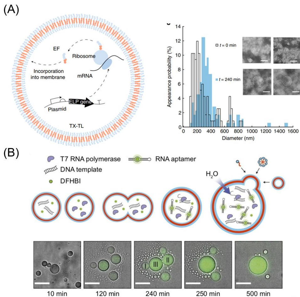
Figure 6. (A) Schematic image of IVTT agents encapsulated ELP-based vesicles and the incorporation of membrane proteins into membrane (left). Size distribution of ELP-based vesicles at the beginning of IVTT and after 240 mins measured by TEM. (right) 96 Adapted with permission from ref (96). Copyright 2018 Kilian Vogele et al. (B) Schematic image of ELP vesicles fusion and expression of dBroccoli RNA aptamers (top) and microscopy image of growing ELP vesicles (bottom) 70 Adapted with permission from ref (70). Copyright 2020 Tobias Pirzer et al.
