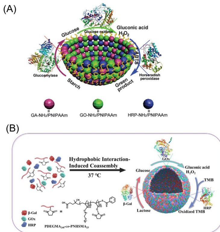
Figure 7. (A) Schematic image of a proteinosome membrane-mediated enzyme cascade reaction. 98 Adapted with permission from ref (98). Copyright 2014 The Royal Society of Chemistry. (B) Schematic image of preparation of multienzyme proteinosomes and enzyme cascade reaction. 99 Adapted with permission from ref (99). Copyright 2021 Elsevier.
