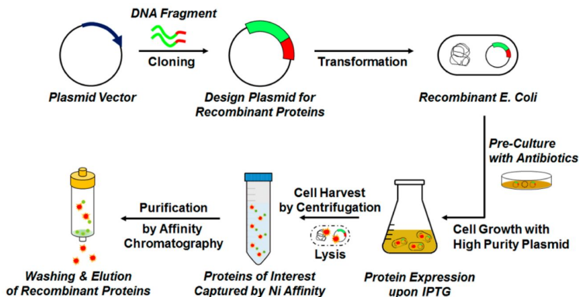
Figure 1. Schematic image of the recombinant protein expression. 53 Adapted with permission from ref (53). Copyright 2016 American Chemical Society
