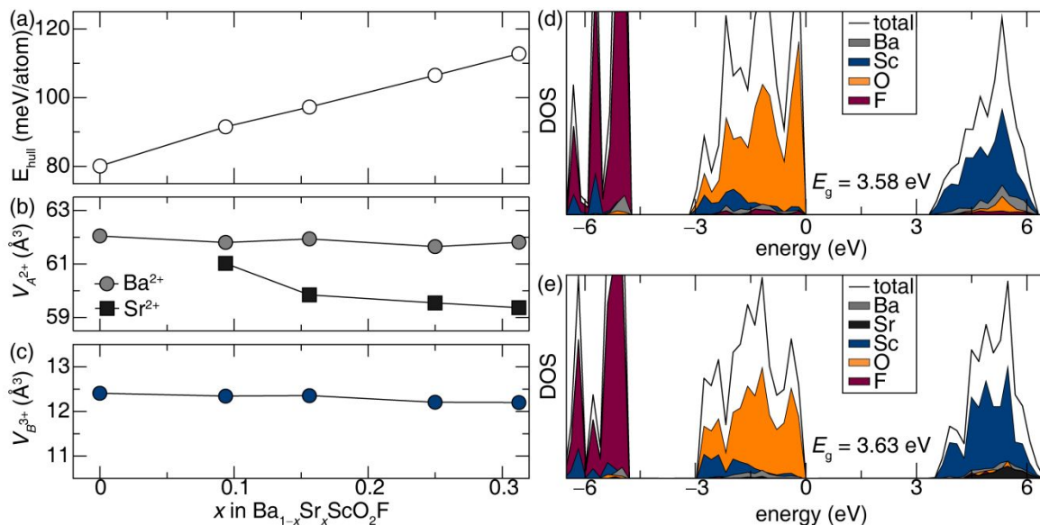
Figure 2. (a) The DFT computed E_{hull} in \text{Ba}_{1-x}\text{Sr}_x\text{ScO}_2\text{F} , where x = 0, 0.09375, 0.15625, 0.25, 0.3125 . The computed polyhedron volume change around (b) \text{Ba}^{2+} and \text{Sr}^{2+} , the A^{2+} site, and (c) \text{Sc}^{3+} , the B^{3+} site, as a function of x . The element-projected density of states of (d) \text{BaScO}_2\text{F} and (e) \text{Ba}_{0.6875}\text{Sr}_{0.3125}\text{ScO}_2\text{F} show a relatively unchanging band gap upon \text{Sr}^{2+} insertion.
