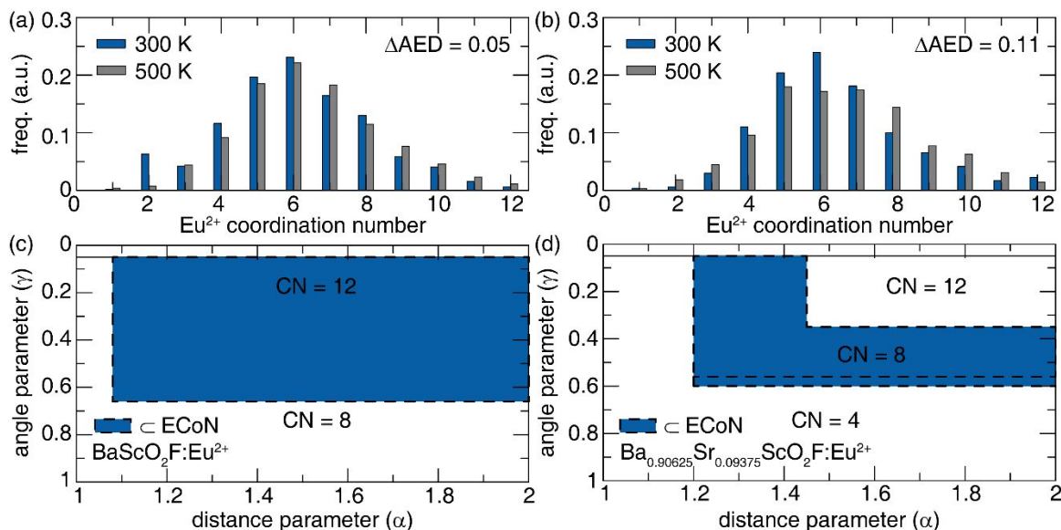
Figure 5. The \text{Eu}^{2+} coordination environment distribution (AED) when (a) x = 0 and (b) x = 0.09375 in \text{Ba}_{1-x}\text{Sr}_x\text{ScO}_2\text{F}:\text{Eu}^{2+} at 300 K (blue) and 500 K (grey). The Voronoi grid representation of \text{Eu}^{2+} local environment of (c) \text{BaScO}_2\text{F}:\text{Eu}^{2+} and (d) \text{Ba}_{0.90625}\text{Sr}_{0.09375}\text{ScO}_2\text{F}:\text{Eu}^{2+} .
