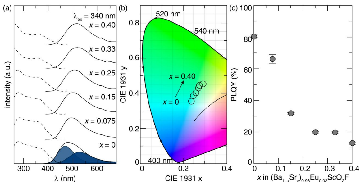
Figure 3. (a) Excitation spectrum (dashed line) and emission spectrum (solid line) where the two blue Gaussian peaks represent the emission from two crystallographically independent \text{Eu}^{2+} sites, (b) CIE coordinates, and (c) room temperature PLQY of (\text{Ba}_{1-x}\text{Sr}_x)_{0.98}\text{Eu}_{0.02}\text{ScO}_2\text{F} ( x = 0.075, 0.15, 0.25, 0.33 , and 0.40 ).
