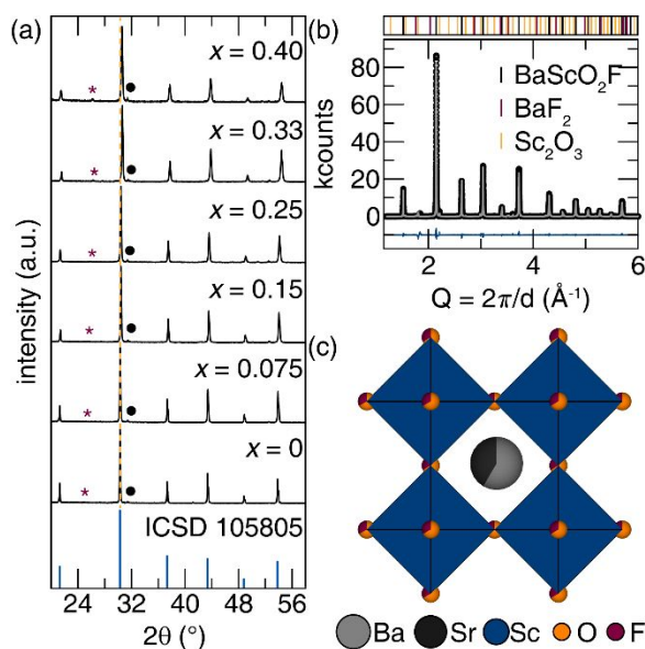
Figure 1. (a) Powder X-ray diffractograms of (\text{Ba}_{1-x}\text{Sr}_x)_{0.98}\text{Eu}_{0.02}\text{ScO}_2\text{F} ( x = 0, 0.075, 0.15, 0.25, 0.33, 0.40 ). \text{BaF}_2 and \text{Sc}_2\text{O}_3 impurities are marked with a red asterisk and a black dot, respectively. (b) Synchrotron refinement of \text{Ba}_{0.566(2)}\text{Sr}_{0.433(8)}\text{ScO}_2\text{F} . The impurity phases were included in the refinement; the refined mole fractions of both impurity phases were less than 5 mol%. (c) The refined perovskite crystal structure of \text{Ba}_{0.566(2)}\text{Sr}_{0.433(8)}\text{ScO}_2\text{F} .
