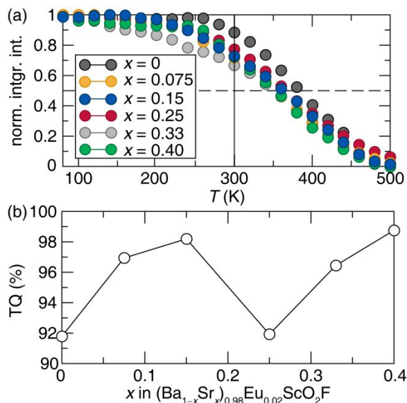
Figure 4. (a) The normalized, integrated emission intensity as a function of temperature from 80 – 500 K and (b) the thermal quenching (TQ) of (\text{Ba}_{1-x}\text{Sr}_x)_{0.98}\text{Eu}_{0.02}\text{ScO}_2\text{F} ( x = 0, 0.075, 0.15, 0.25, 0.33, 0.40 ) expressed as the ratio between the integrated light intensity emitted at 500 K and 300 K.
