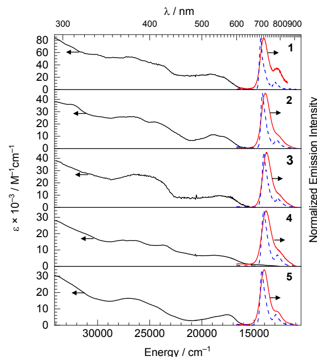
Fig. 2. Stacked plots of UV-Vis absorption and room temperature PL emission spectra were measured in deaerated THF (black and red solid lines), along with 77 K PL emission spectra measured in toluene glass (blue dashed lines).
