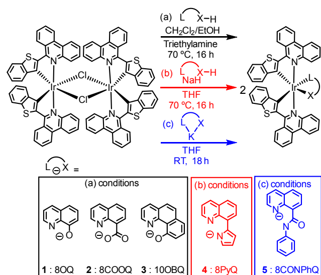
Scheme 1. Synthesis of iridium complexes described here.
