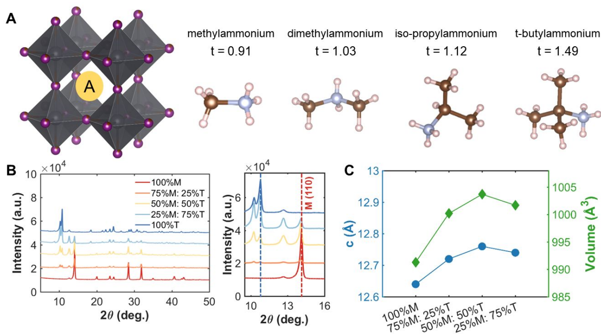
Figure 1. Crystallographic features of the perovskites studied. A. Various A -site cations (M, D, I, and T) with their tolerance factors. The single crystal structures for D, I, and T are shown in supporting information Figure S1. B. The peak shift shown on M-T series in the thin-film form.
