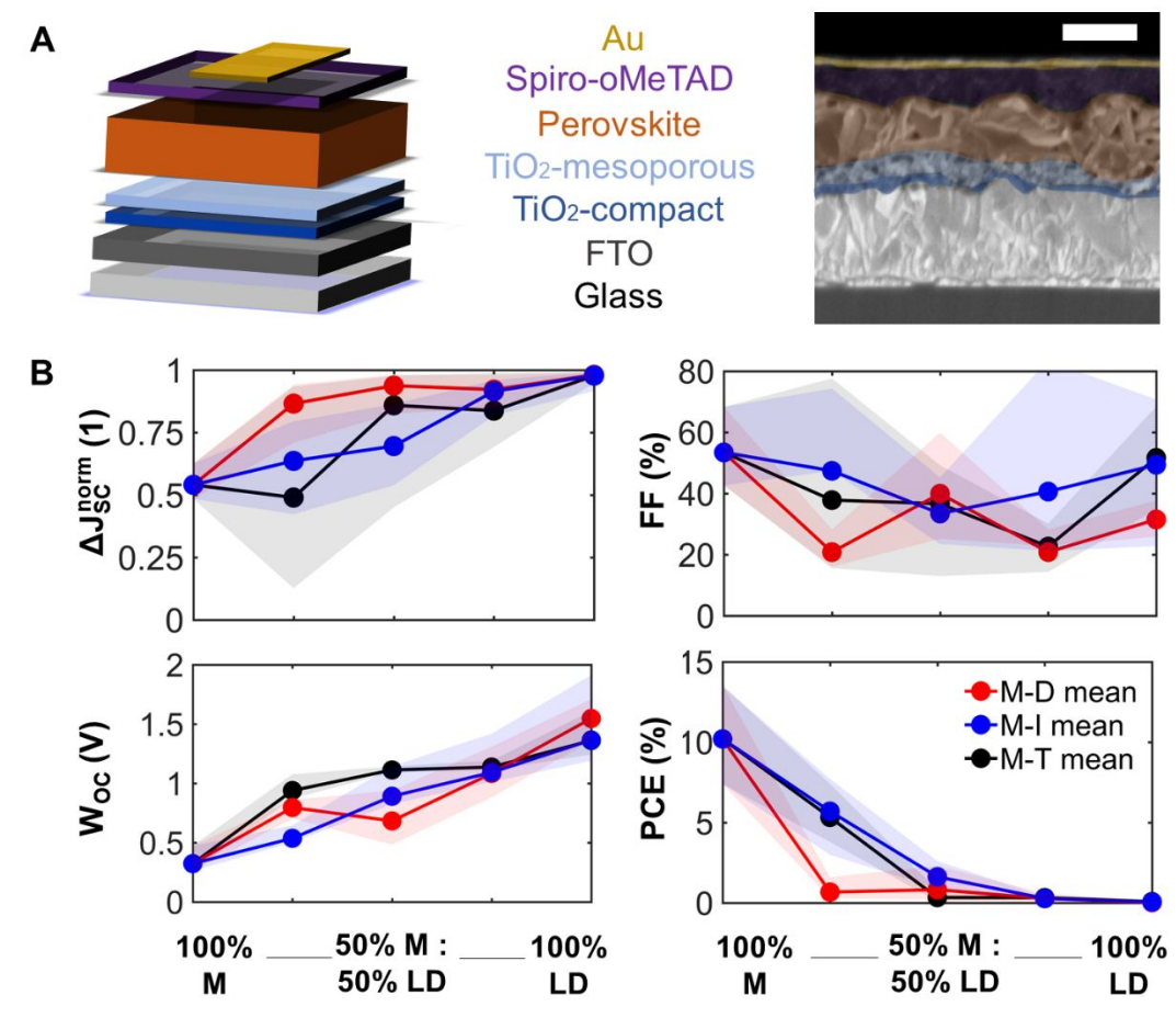
Figure 3. Solar cell performance parameters of the 3D/LD mixed perovskites. A. A schematic and a SEM image (artificially colored) for the device stack of 25% M : 75% T device, 500 nm scale bar. B. The plot and average of solar cell performance metrics for M-D, M-I, and M-T series, including \Delta J_{SC}^{norm} (short-circuit current density deficit normalized), calculated by normalizing the difference between the theoretical maximum bandgap-specific J_{SC} with the measured J_{SC} , W_{OC} (bandgap-voltage offset at open-circuit condition), calculated by subtracting the Shockley-
