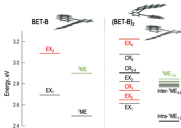
Fig. 12 Energy levels of BET-B (left) and (BET-B) 2 (right) computed at the RAS-SF/cc-pVDZ level. Energies were corrected by means of excited state decomposition analysis 80 . Dark, bright, t and quintet states marked in black, red and green, respectively. EX: excitonic state; CR: charge resonance; ME: multiexcitonic state.
