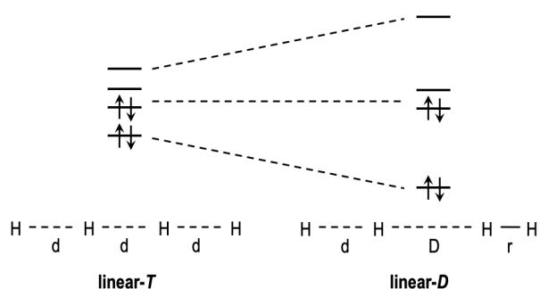
Fig. 9 Molecular orbital diagrams (top) and the structures (bottom) of the model H 4 system in two linear arrangements with tetradical (left: linear- T ) and diradical (right: linear- D ) character. Interatomic distances: d = 3.0 \text{ \AA} ; D = 7.0 \text{ \AA} ; r = 0.743 \text{ \AA} .
