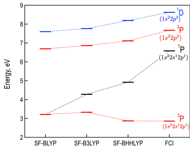
Fig. 5 Low-lying electronic states of Be computed with FCI and SF-TDDFT with GGA functionals with different amounts of the exact exchange: 0% (BLYP), 20% (B3LYP), and 50% (BHHLYP), and the 6-31G basis set.
