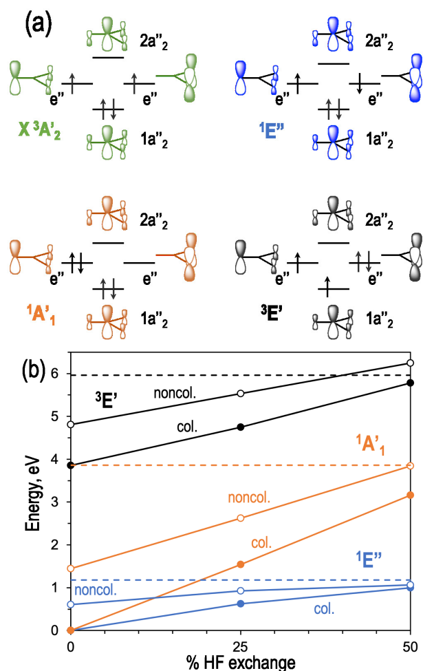
Fig. 6 (a) Molecular orbital diagram for the ground ( X^3A'_2 ) and low-lying electronic states ( {}^1E'' , {}^1A'_1 , and {}^3E' ) of the TMM diradical. (b) Collinear (full circles) and non-collinear (empty circles) SF-TDDFT/TDA vertical transition energies of TMM computed with the PBE xc functional mixed with different amounts of HF exchange and the cc-pVTZ basis set. Dashed lines indicate the reference values obtained with SF-OD. 38
