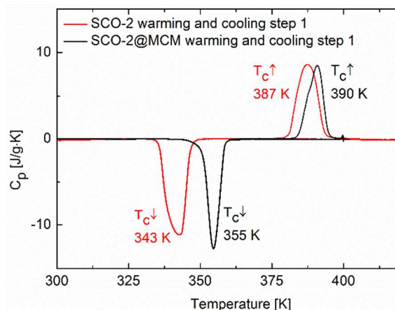
Fig. 13 Heat capacity versus temperature for SCO-2 and SCO-2@MCM recorded by differential scanning calorimetry at 10 K/min.
