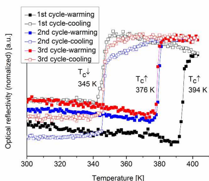
Fig. 11 Thermal dependence of the normalized optical reflectivity of SCO-1@MCM at a scan rate of 2 K/min. The transition temperatures recorded in warming and cooling modes are indicated.
