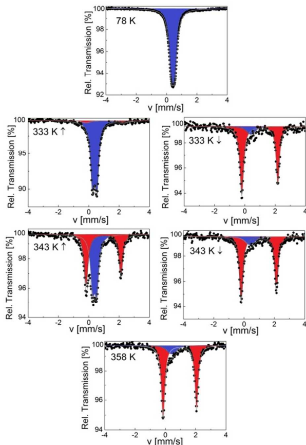
Fig. 9 Selected ^{57}\text{Fe} Mössbauer spectra of SCO-2@MCM; red and blue colors correspond to HS and LS doublets, respectively.
