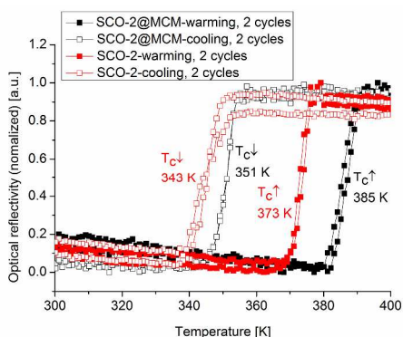
Fig. 12 Thermal dependence of the normalized optical reflectivity recorded at 2 K/min on both SCO-2@MCM (black curves) and SCO-2 prepared as nanoparticles (red curves) using the reverse micelle method. The transition temperatures in the warming and cooling modes are given.
