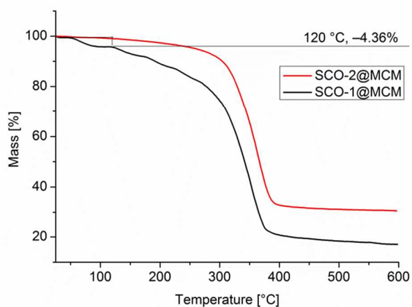
Fig. 14 Thermogravimetric analysis (TGA) shows that SCO-1@MCM possesses crystal water, whereas SCO-2@MCM nearly does not contain solvent. Up to 120 °C, 4.36 and 0.95 wt.% are lost for SCO-1 and SCO-2@MCM, respectively. 4.36 wt.% correlated to a Fe content of 7.2 wt.% correspond to about 2 \text{H}_2\text{O} molecules per SCO-1 formula unit (that is per Fe atom) in SCO-1@MCM. Further heating shows that the SCO-1@MCM composite contains more water which is lost above 120 °C.
