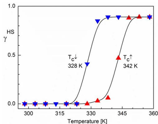
Fig. 8 Temperature dependence of the HS molar fraction ( \gamma^{\text{HS}} ) deduced from ^{57}\text{Fe} Mössbauer spectroscopy over the temperature range 298-360 K for SCO-1@MCM (top) and for SCO-2@MCM (bottom).
